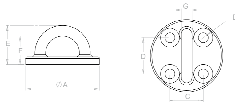
Golfare rotondo Classical Pad-eye
