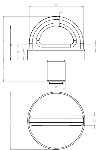
Golfare girevole Revolving Pad-eye
