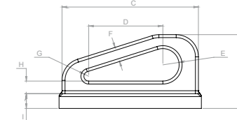
Golfare laterale Lateral Pad-eye
